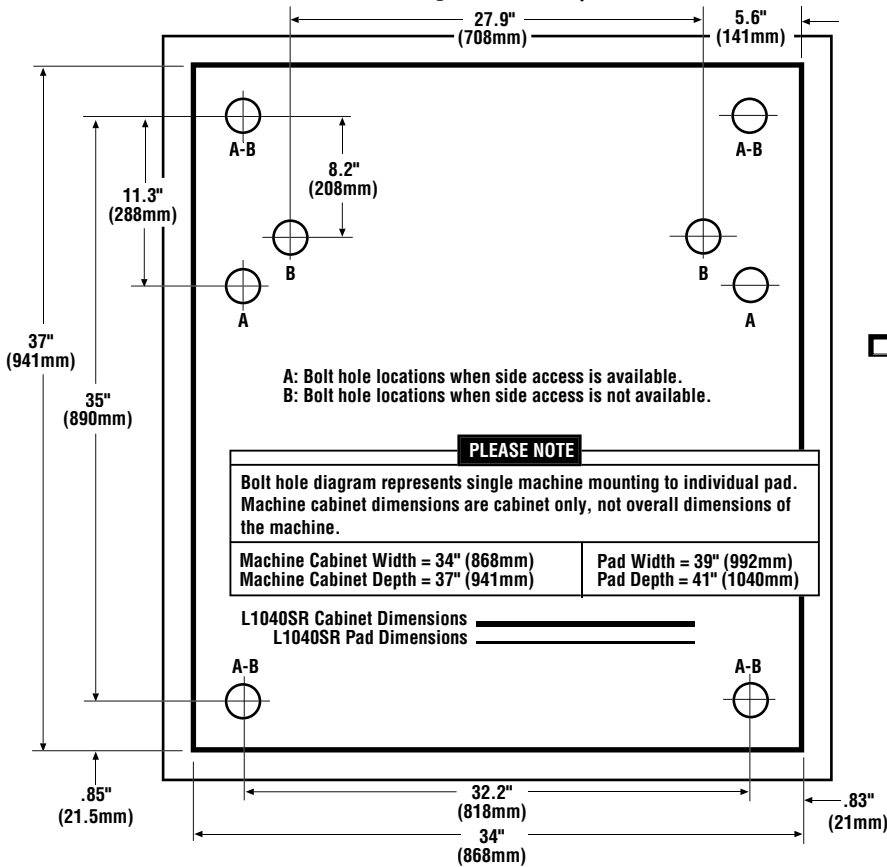
Machine Front
